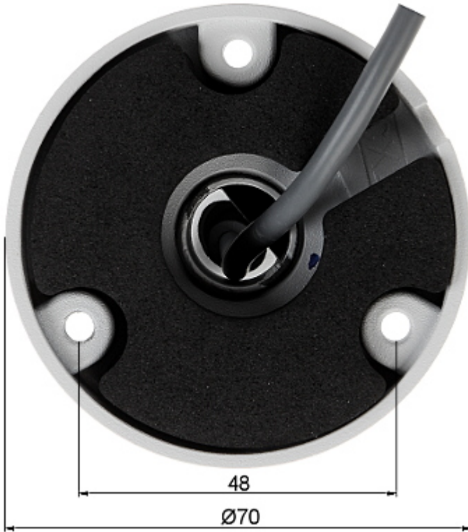
Camera dimensions:
