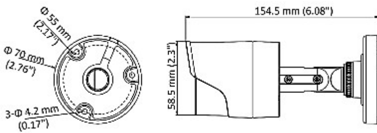
Camera dimensions:
