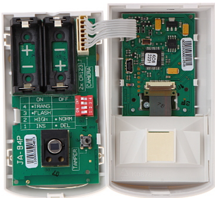
Mounting side view + additional elements included in the kit:
