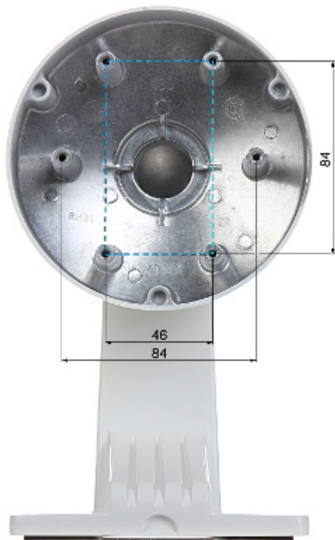
Wall mounting side view:
