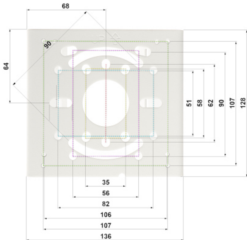
Top view - clamping strips diameters range:
