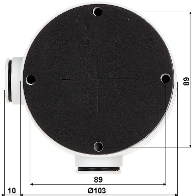
Camera dimensions:
