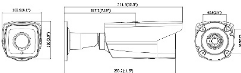
Camera dimensions:
