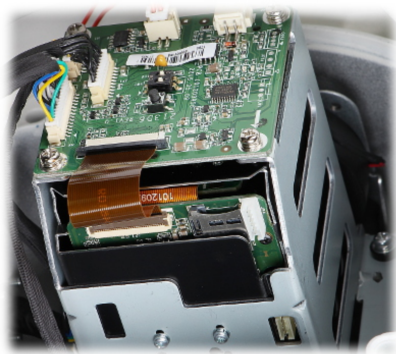
Camera connectors:
