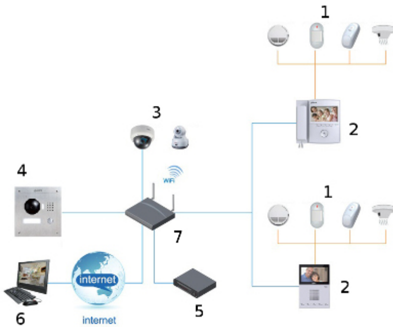
Connection diagram:
