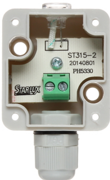
Connection diagram:
