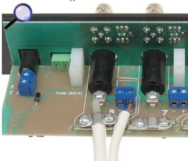
Connection of the YAP type cable:
