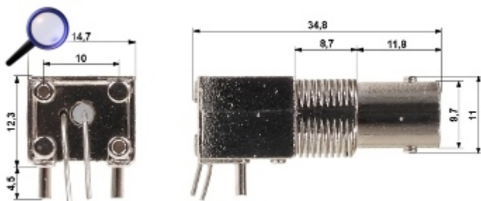
Socket dimensions:
