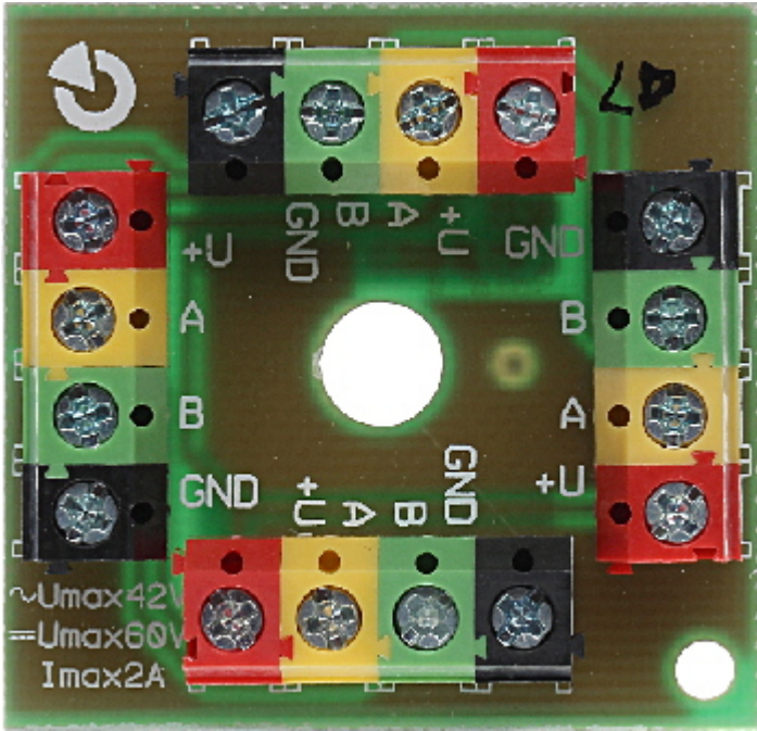
Device connectors:
