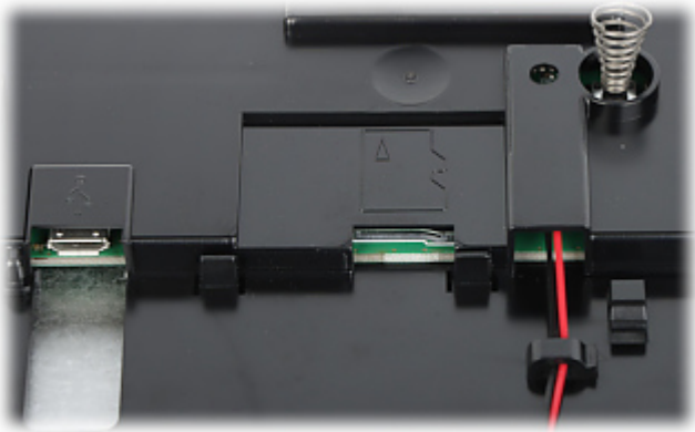
Keyboard connectors:
