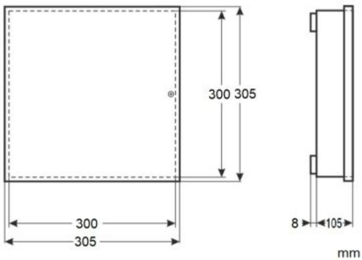
Dimensions:
