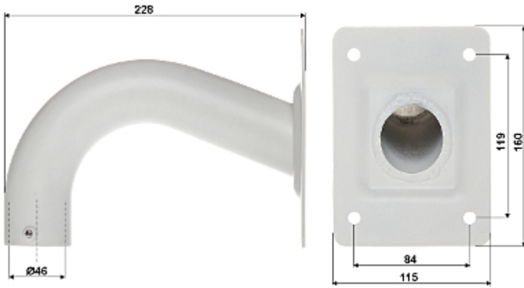
Camera dimensions:
