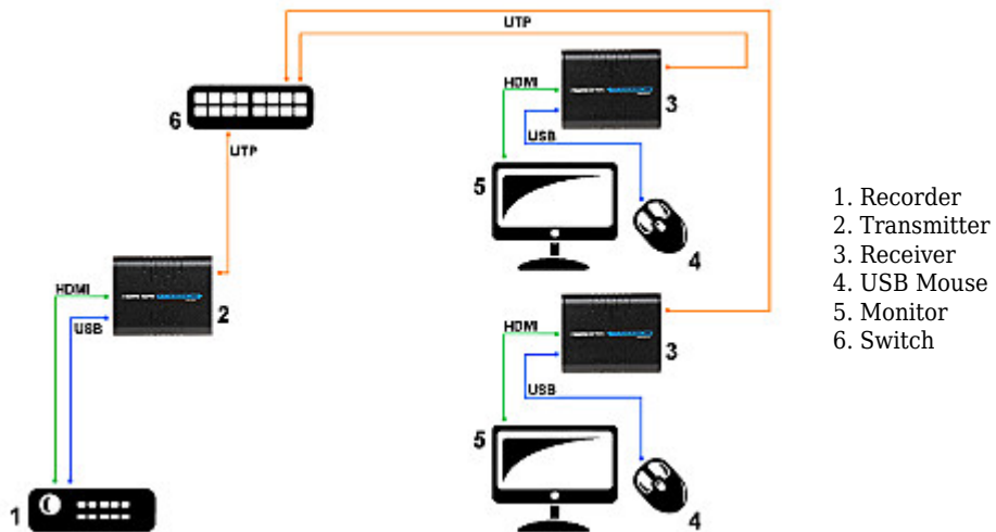
Connection schematic diagram:
