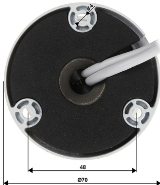
Camera mounting side view:
