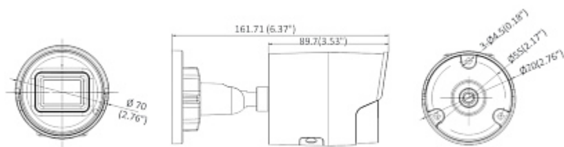
Camera dimensions:
