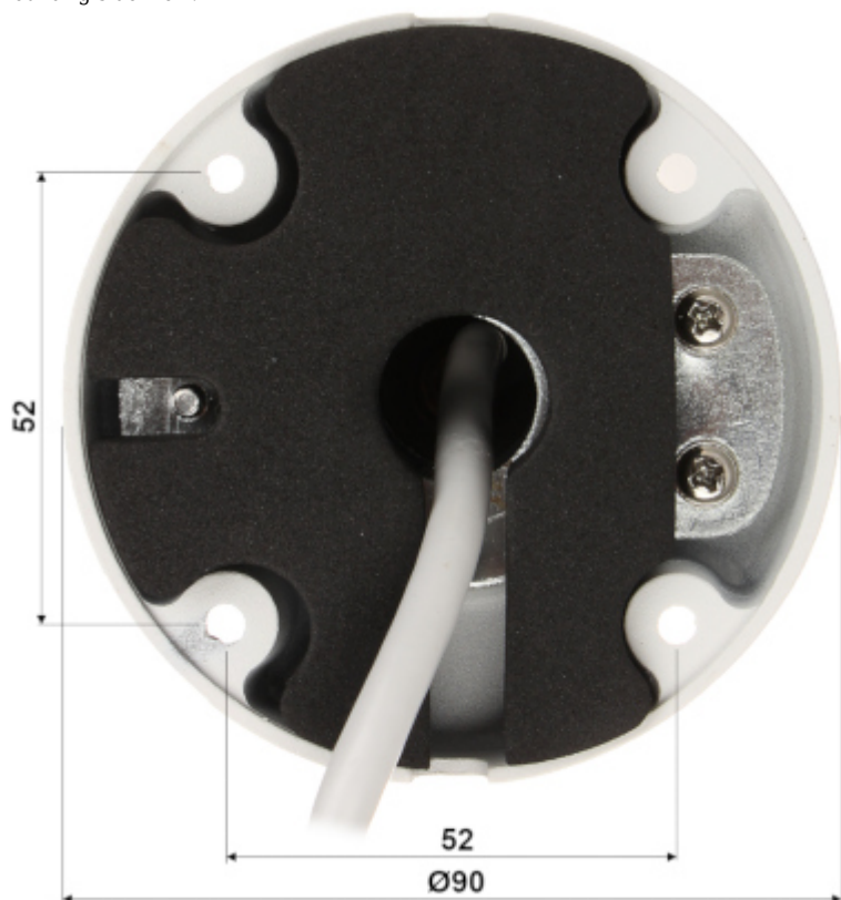
Camera connectors:
