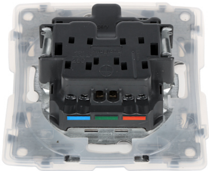
Connectors view:
