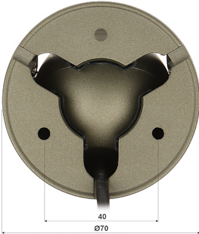
Camera connector:
