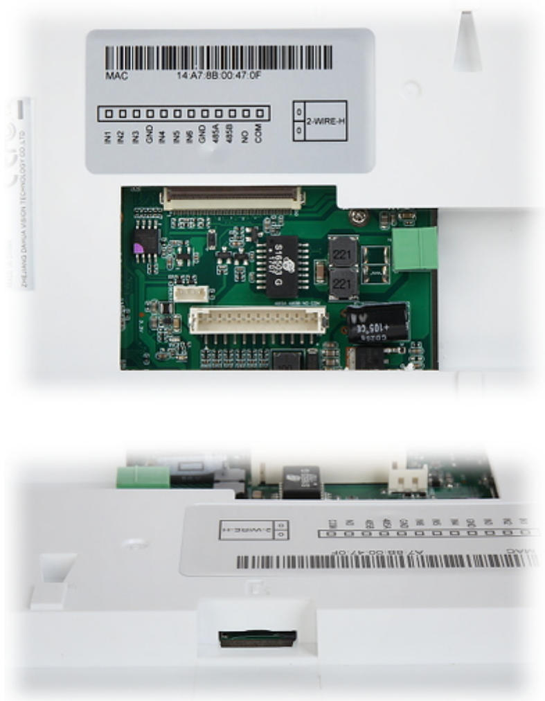
Connectors view:
