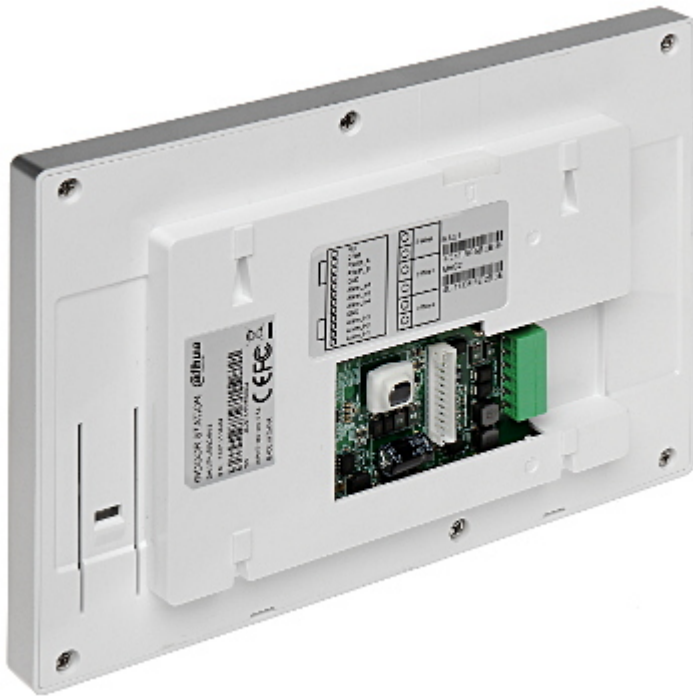
Connectors view:
