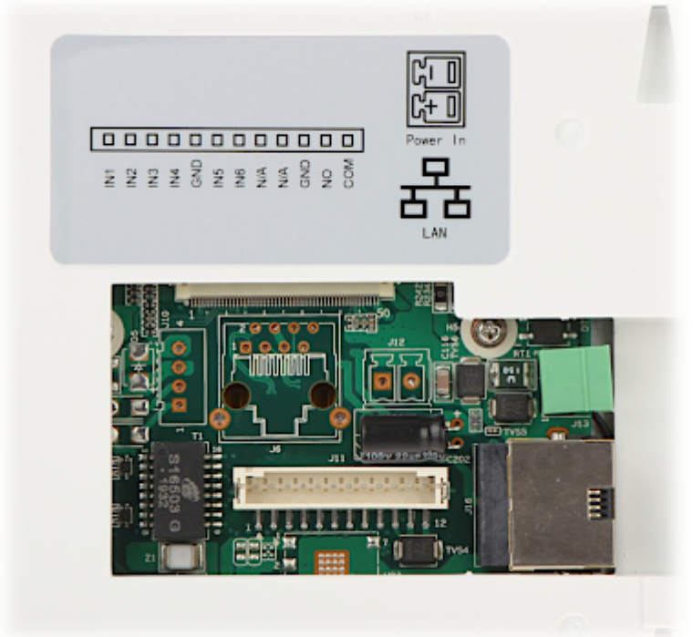
Connectors view:
