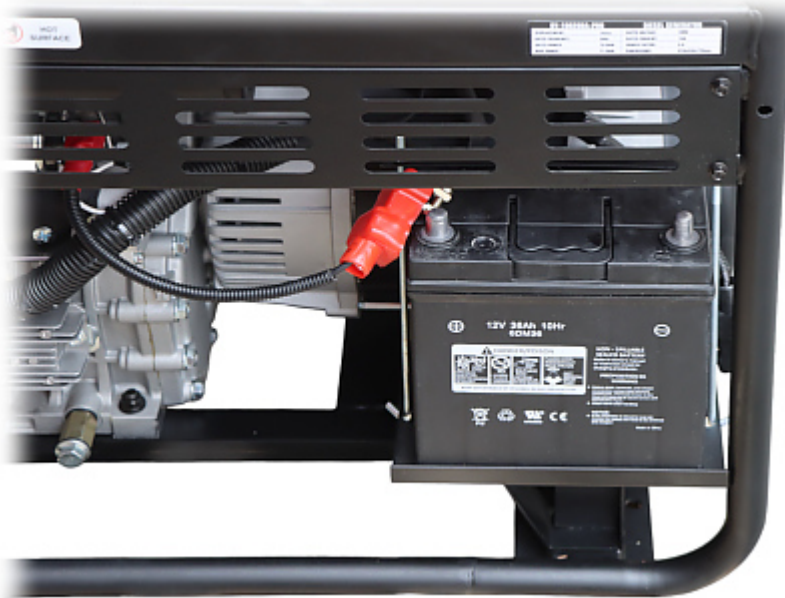
Fuel filler and fuel gauge:
