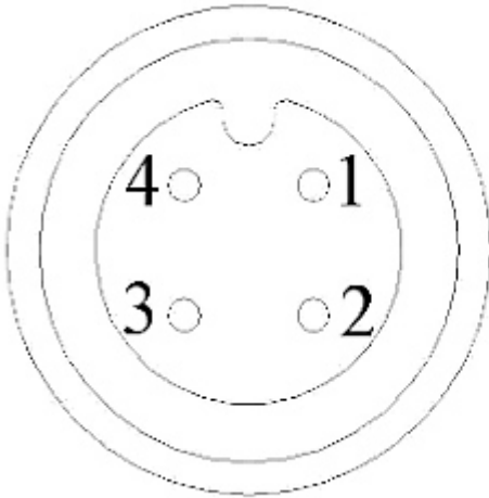
M12 connector:
