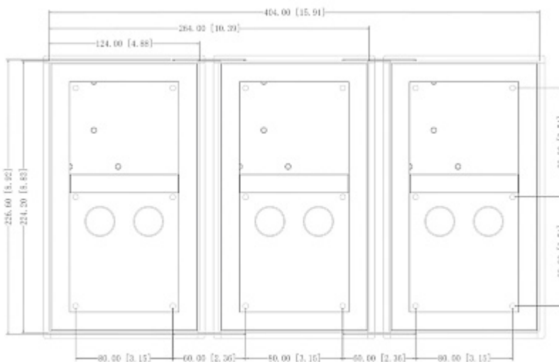
Dimensions with 3 elements combined - back side:
