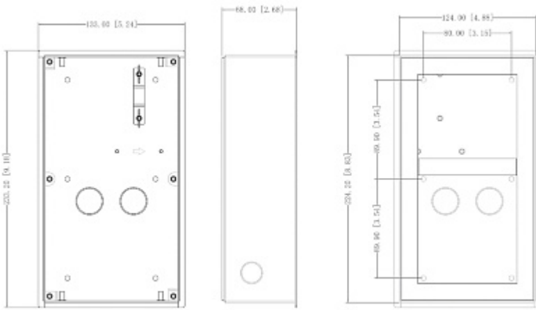
Dimensions with 3 elements combined - front side:
