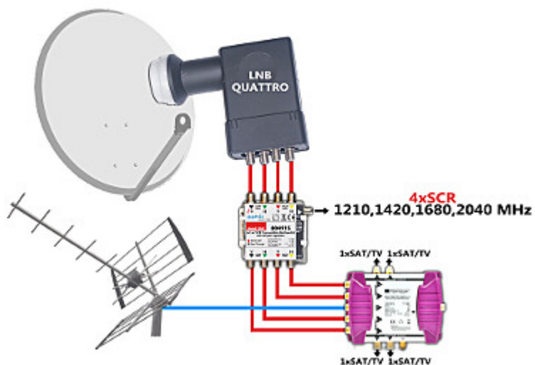
1 - SAT Gain control Example of application:
