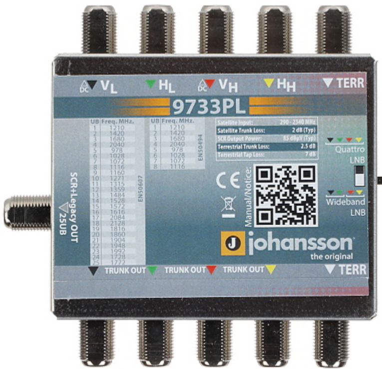
Connectors view:
