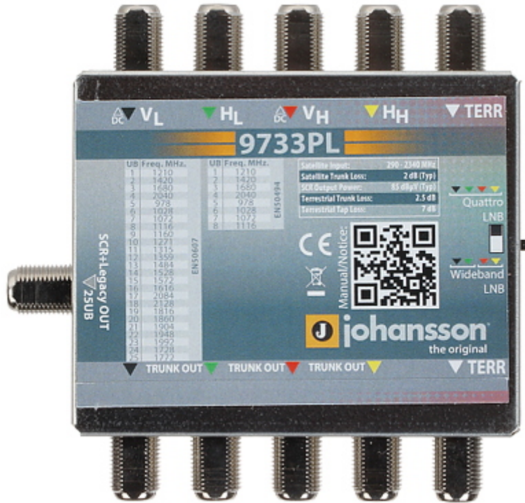
Connectors view:
