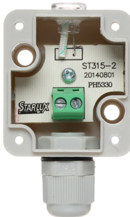
Internal view:
