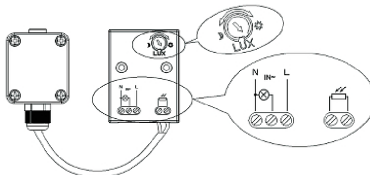
Connection diagram:
