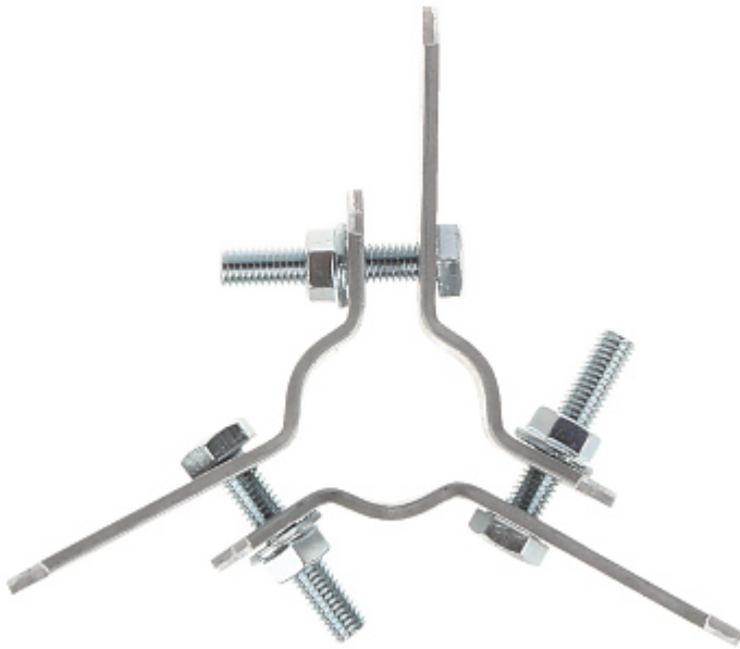
Mast base correctly assembled:
