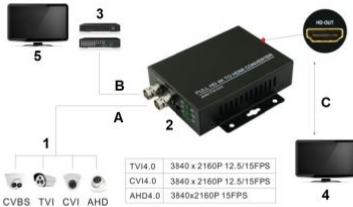
Schematic diagram of converter operation:
