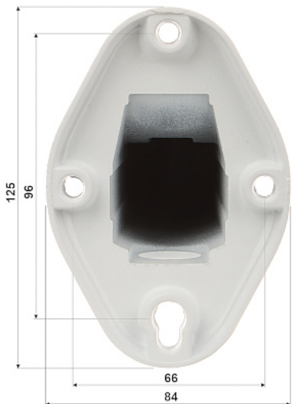
Bracket camera or housing mounting base dimensions:
