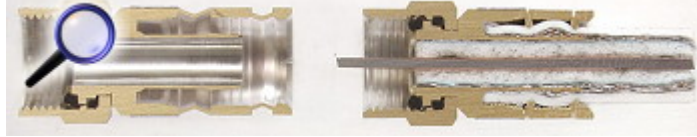
Sectional views of the new and compressed connector on RG-6 cable:
