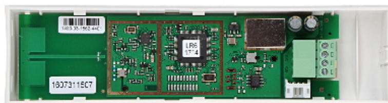
Internal view of the housing:
