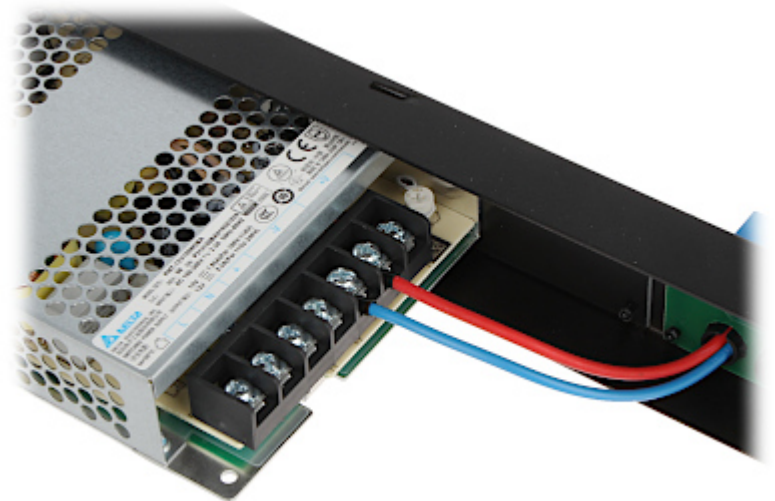
Rear view:
