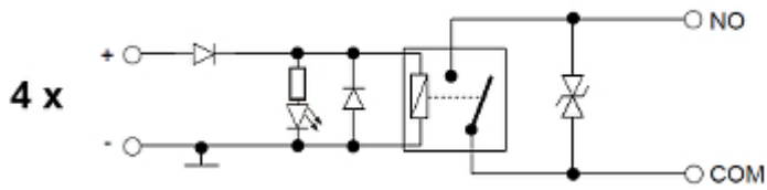
Schematic diagram:
