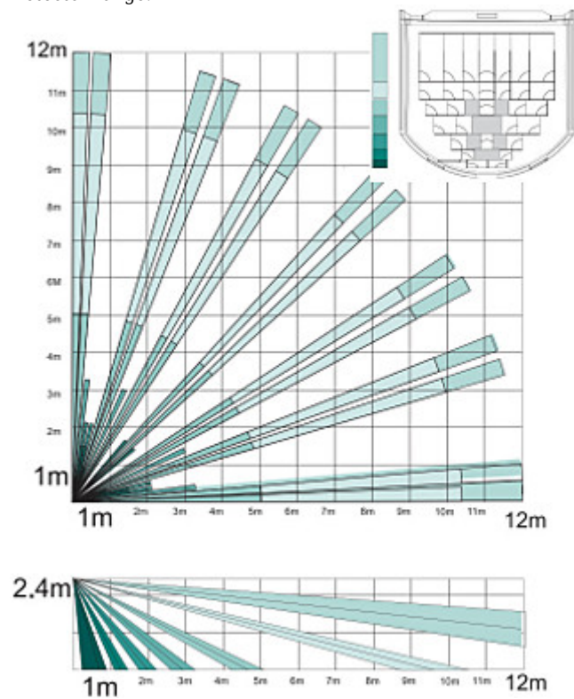
Remote controller:
