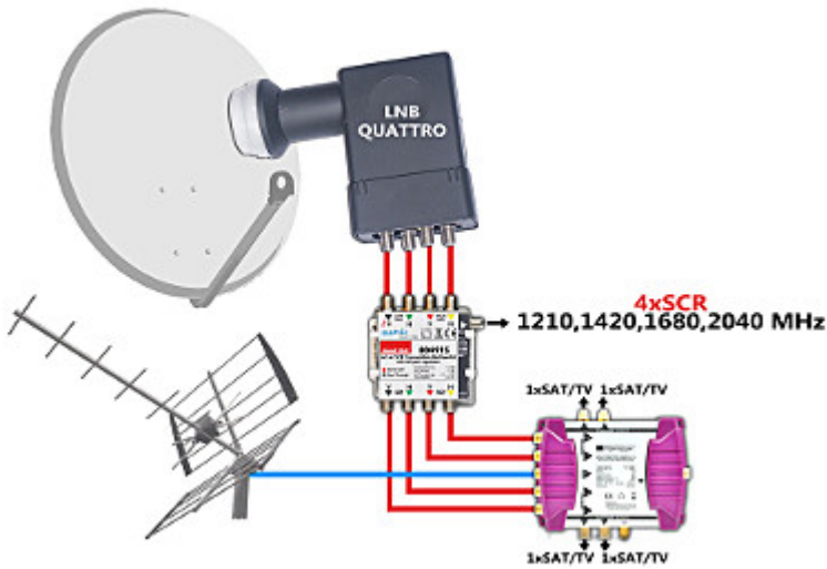
1 - SAT Gain control Example of application:
