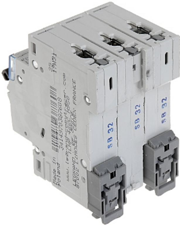
Bottom view:
