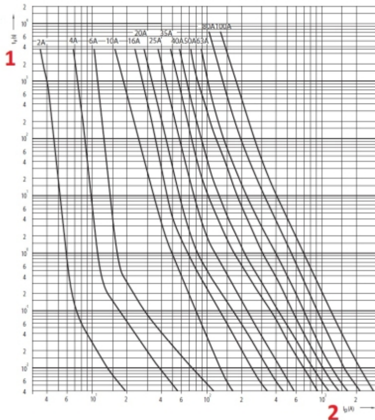
Time-current characteristics:
