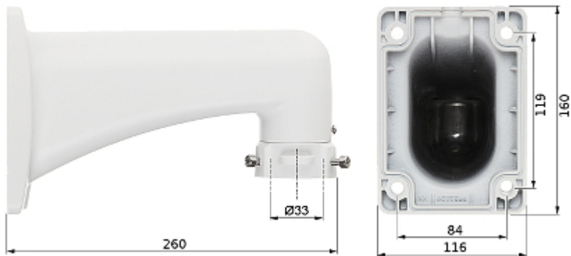
Camera dimensions:
