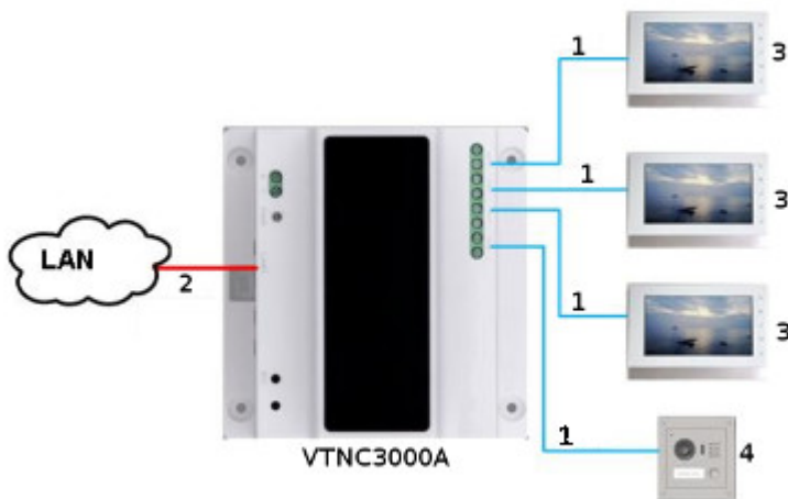
Connection schematic diagram:
