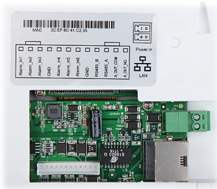
Connectors view:
