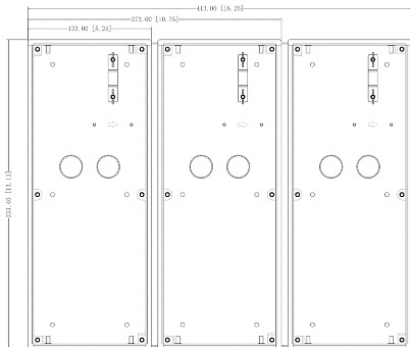
Dimensions with 3 elements combined - back side:
