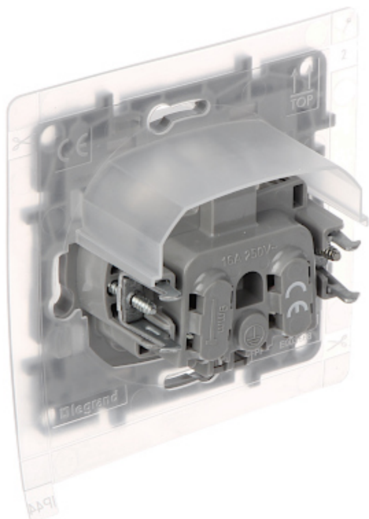
Connectors view:
