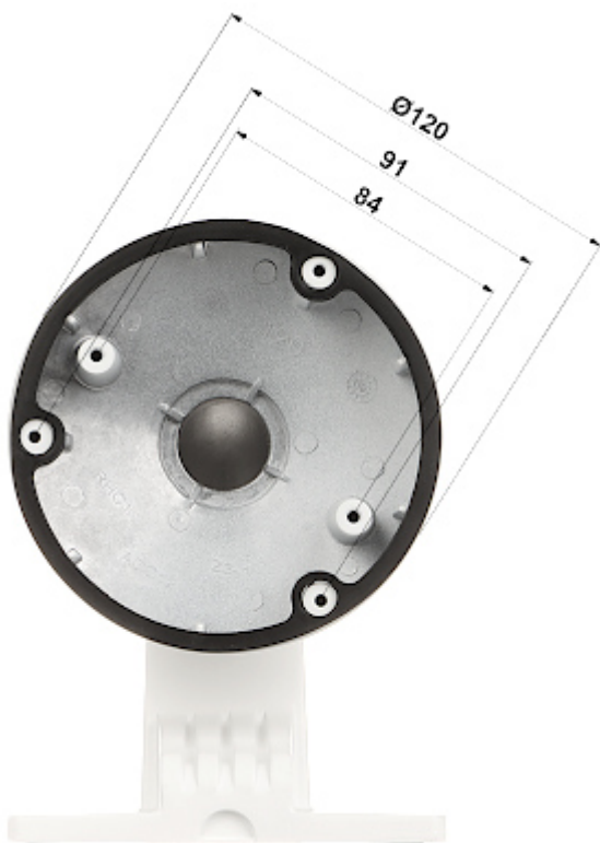
Bracket dimensions:
