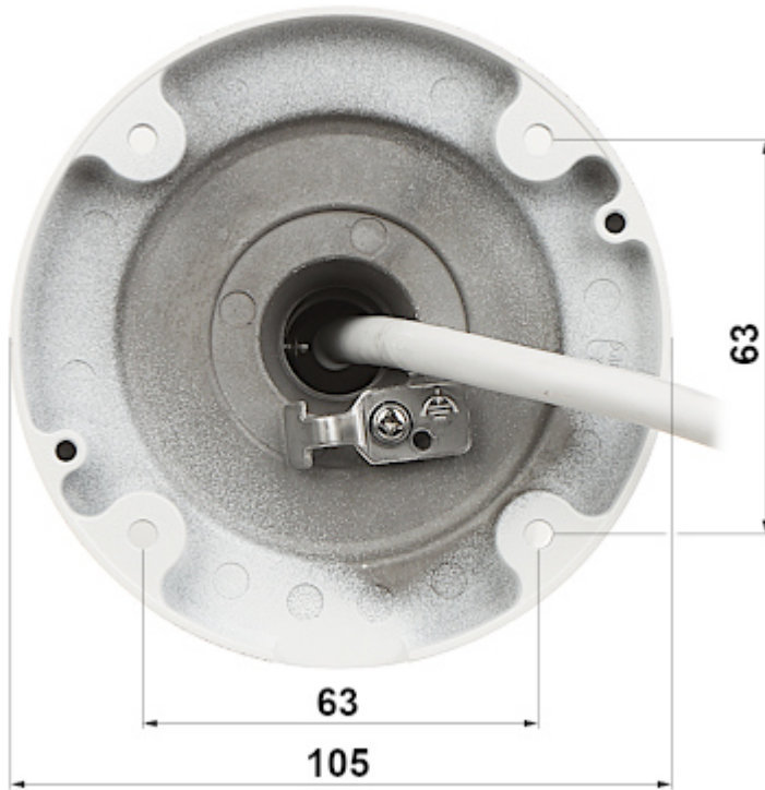
Camera dimensions:
