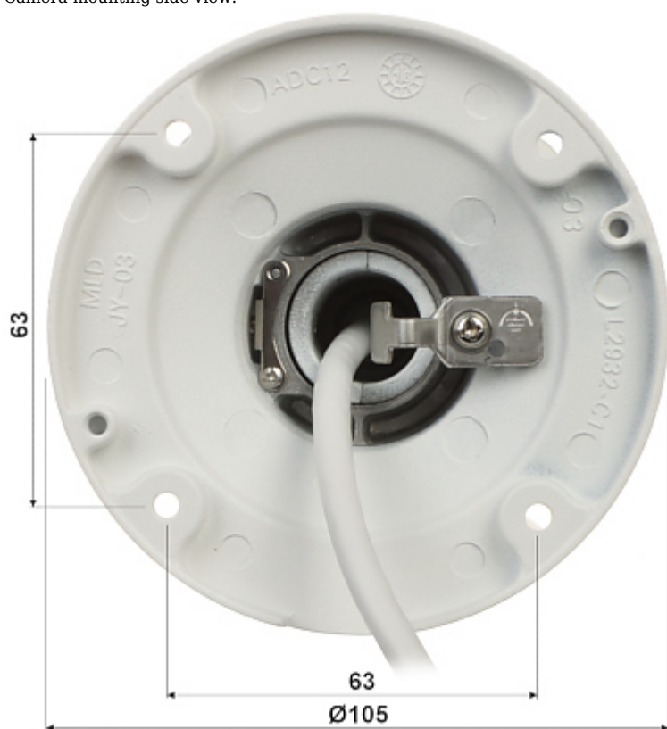
Camera dimensions:
