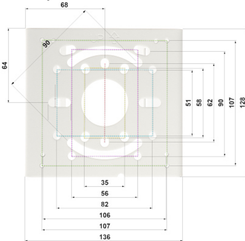
Top view - clamping strips diameters range:
