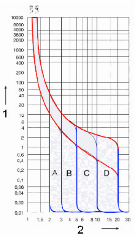
Tripping curves:
